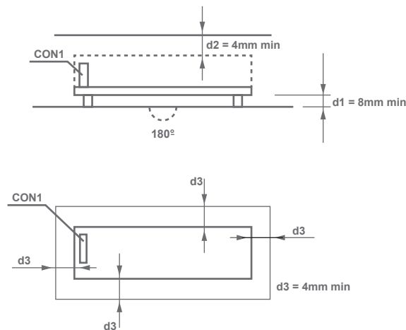
Fig.1.1 Installation method
